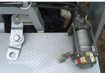
10,000 lbs Line Pull Winch & Pulley
